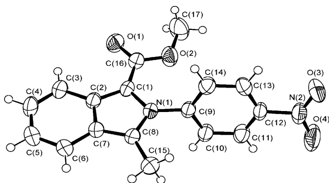
Figure 1. X-ray structure of 3d .
