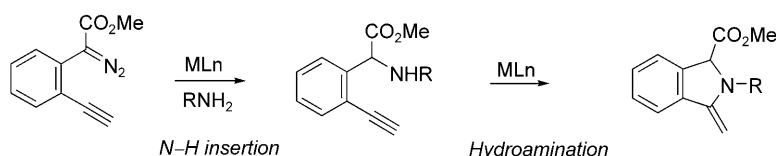
Scheme 1. Two C–N bond formations catalyzed by single catalyst.
